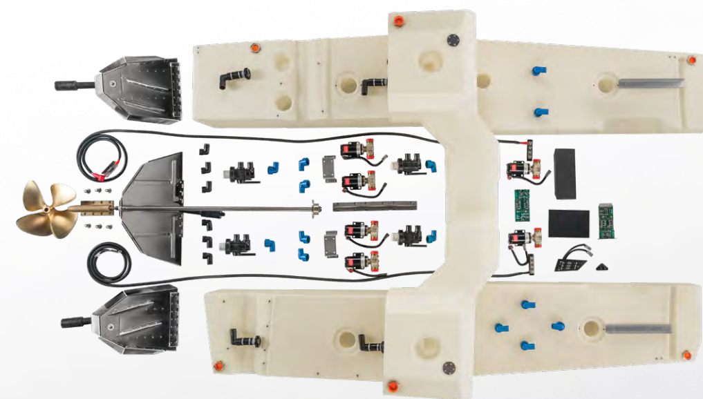
SWITCHBACK BALLAST TANK
